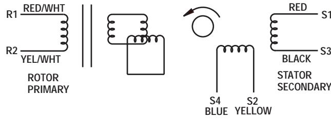
SCHEMATIC DRAWING FOR BRUSHLESS RESOLVER
