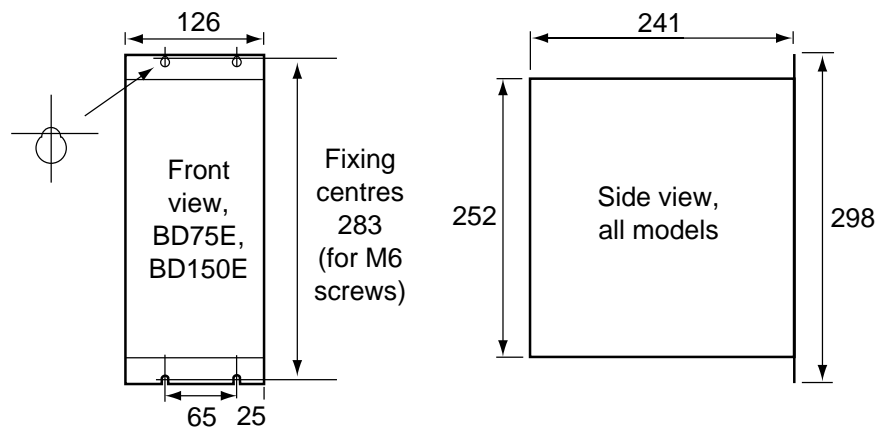
Figure 3-1. Drive Dimensions
