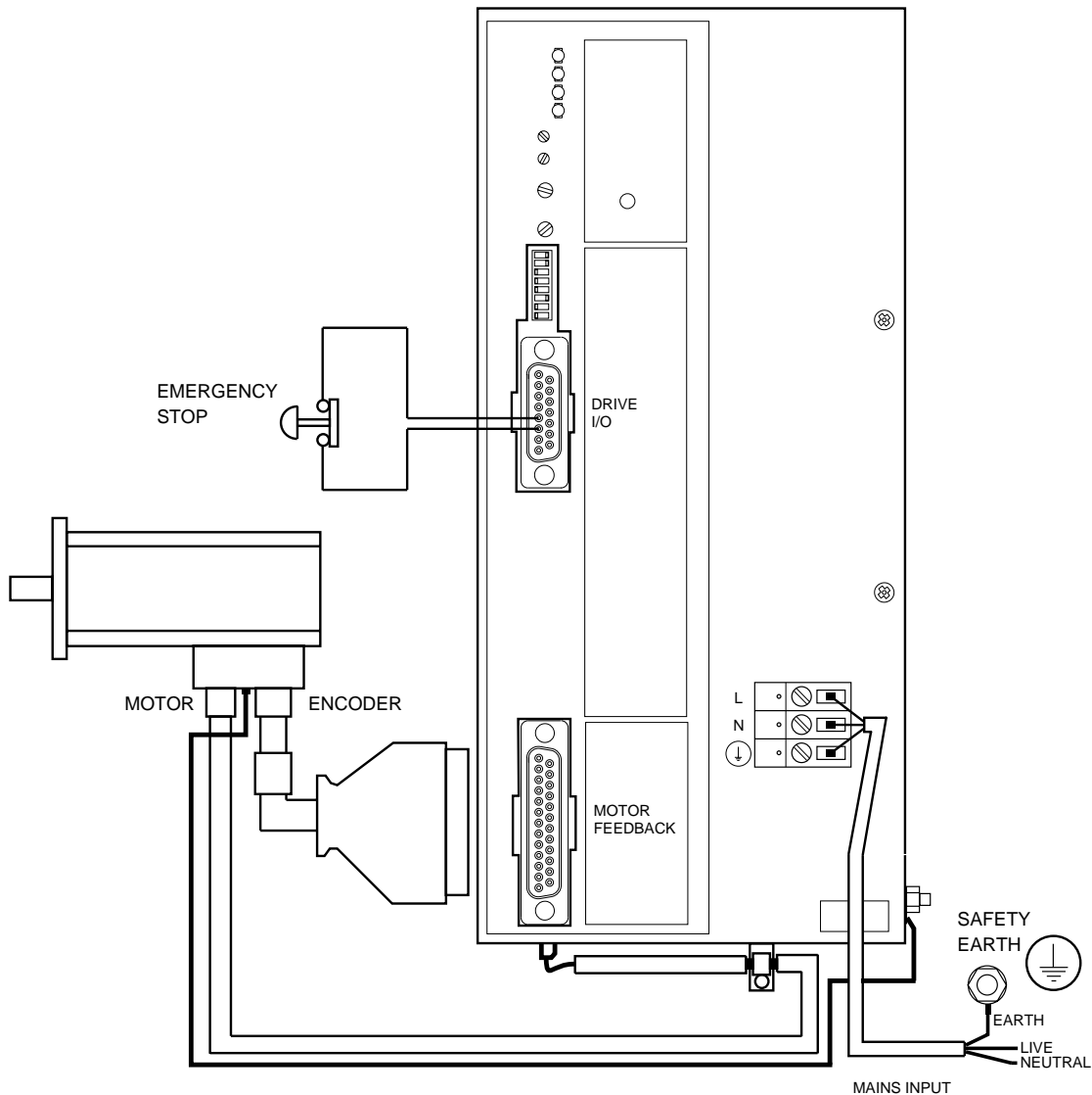
Figure 2-2. Pre-installation Test Configuration
