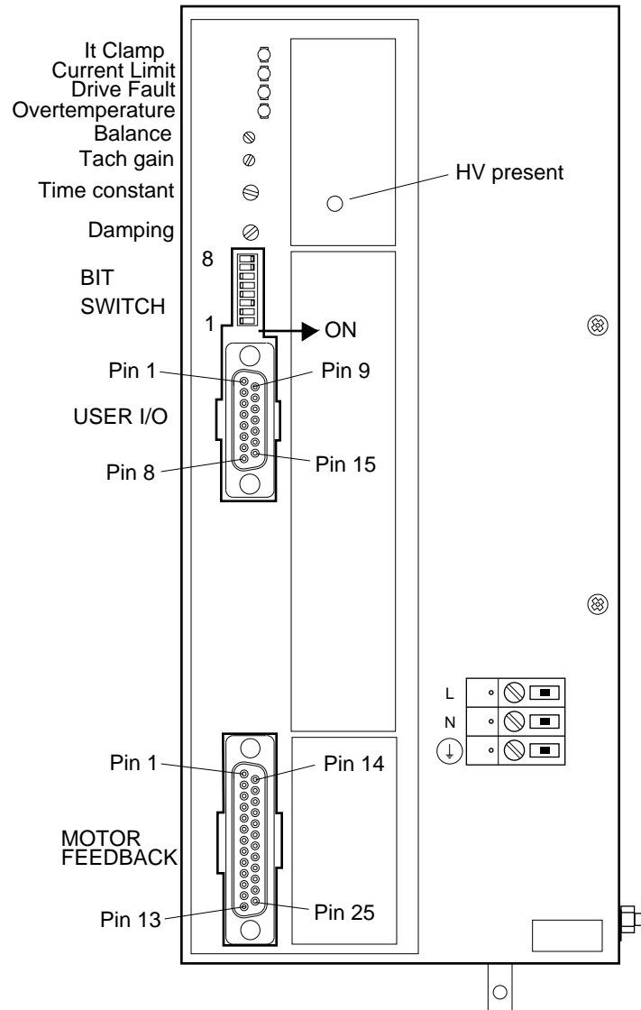
Figure 3-2. Connectors and Indicators
