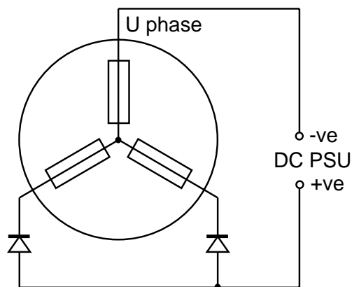
Figure A-1. Encoder Set-up Circuit
