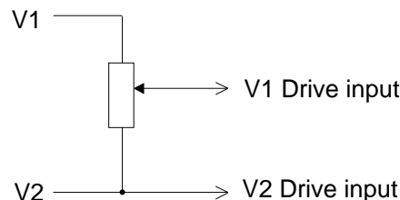
Figure 3-6. Circuit for accurate torque amp gain setting
