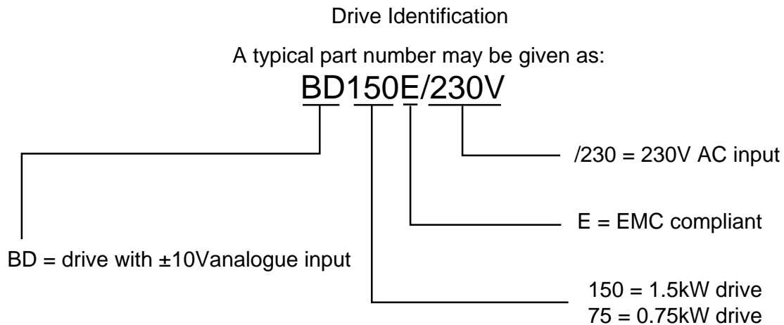
Figure 2-1. Drive Identification
