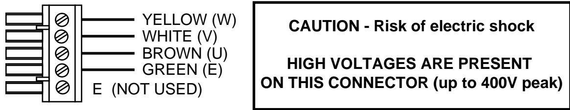
Figure 3-3. Motor Connector
