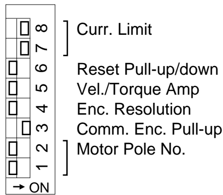
Figure A-2. Bit Switch Settings
