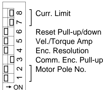
Figure 3-5. Bit Switch Settings
